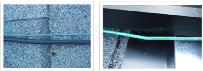
Photo 8: Source circuit conductors in contact with roof: NEC 338.10, 334.30
